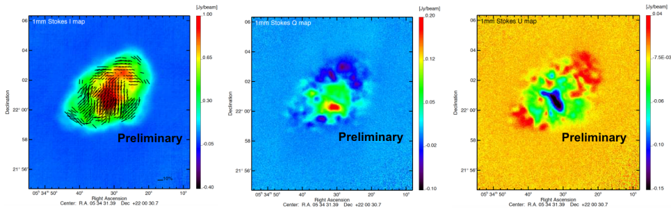
Figure 3. NIKA2 Stokes parameter maps of the Crab Nebula at 1.15 mm. From left to right: intensity map with polarization vectors overlotted where the polarization intensity SNR > 3\sigma , Stokes Q map, and Stokes U map.
