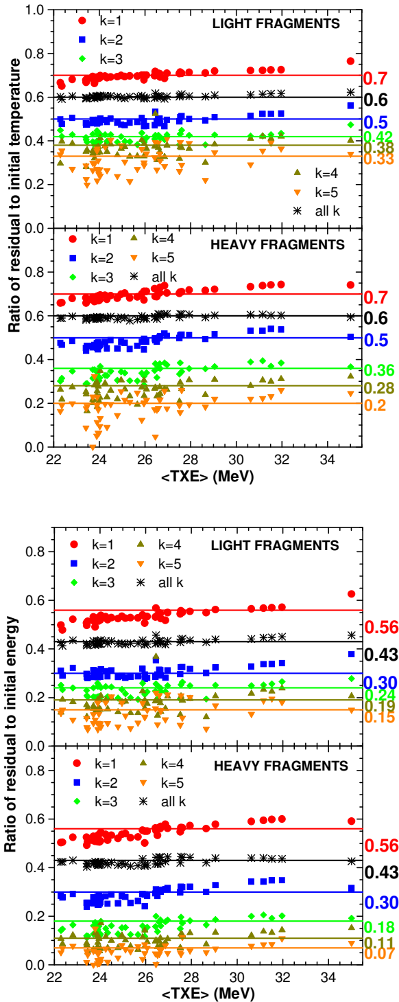
Fig.1: The ratios of residual temperature (upper part) and residual energy (lower part) to those of initial fragments corresponding to each sequence k (different coloured symbols) and to all emission sequences (black stars) and the constant values approximating these ratios (horizontal lines plotted with the same colour as the respective symbol).
