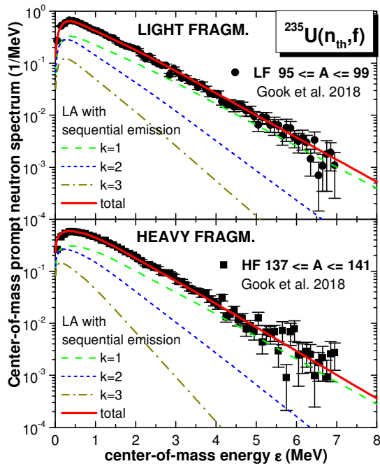
Fig.3: Prompt neutron spectra in the centre-of-mass frame corresponding to the light and heavy fragment group (upper and lower part, respectively): The result of the LA model with sequential emission: \Phi_k(\epsilon) of the first three emitted neutrons (different dashed and dotted lines) and the total \Phi(\epsilon) (red solid line) describing very well the experimental data of Gök et al.[5] (symbols).
