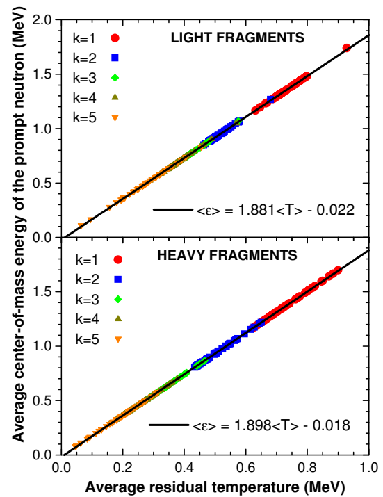
Fig.2: Average centre-of-mass energy of each emitted neutron \langle \varepsilon \rangle_k (different symbols for k from 1 to 5) as a function of the average residual temperature \langle T_k \rangle . The linear fits are given with black lines.
