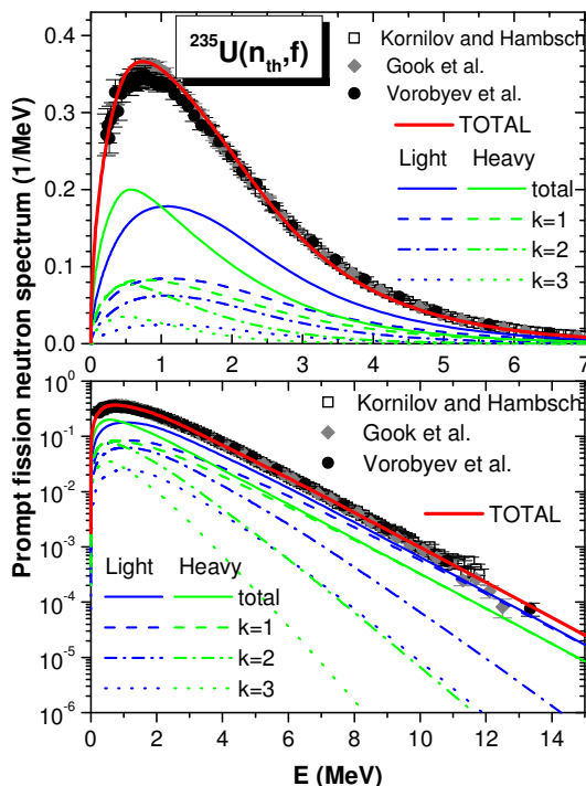
Fig.4: PFNS result of the LA model with sequential emission: spectra of each emitted neutron (different dashed or dotted lines) and of all emitted neutrons (thin solid lines) from the light (blue colour) and heavy (green colour) fragments and the total spectrum (thick solid red line) describing well the experimental data (different symbols).
