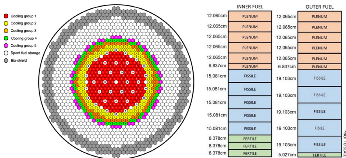
Figure 2: Radial mesh according to cooling group distribution and axial mesh layers
