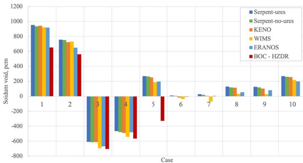
Figure 6: Sodium void effect results
