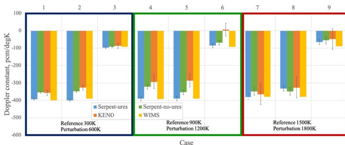
Figure 4: Doppler results
