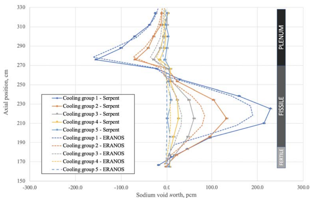
Figure 8: Local sodium void effect results
