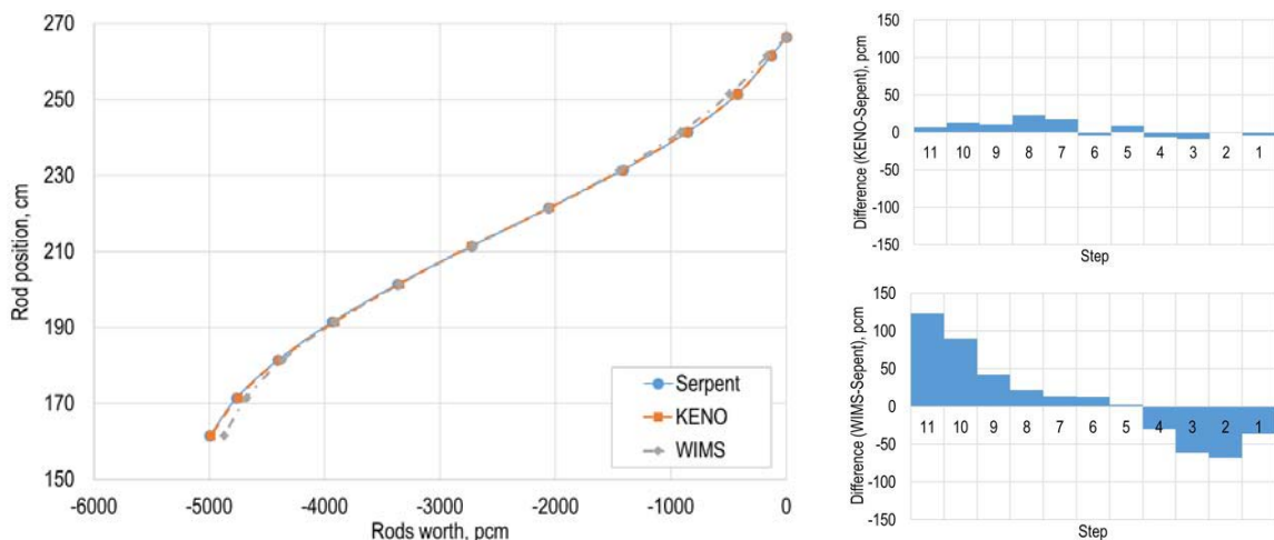
Figure 3: Control rod worths and differences between KENO-VI/WIMS and Serpent
