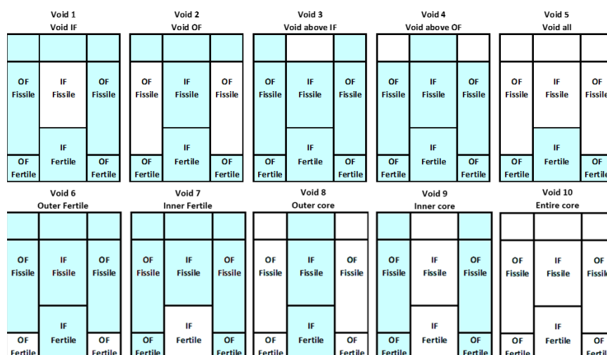
Figure 1: Sodium void zones and corresponding case numbers
