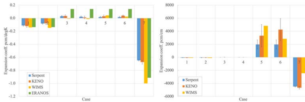
Figure 5: Thermal expansion results
