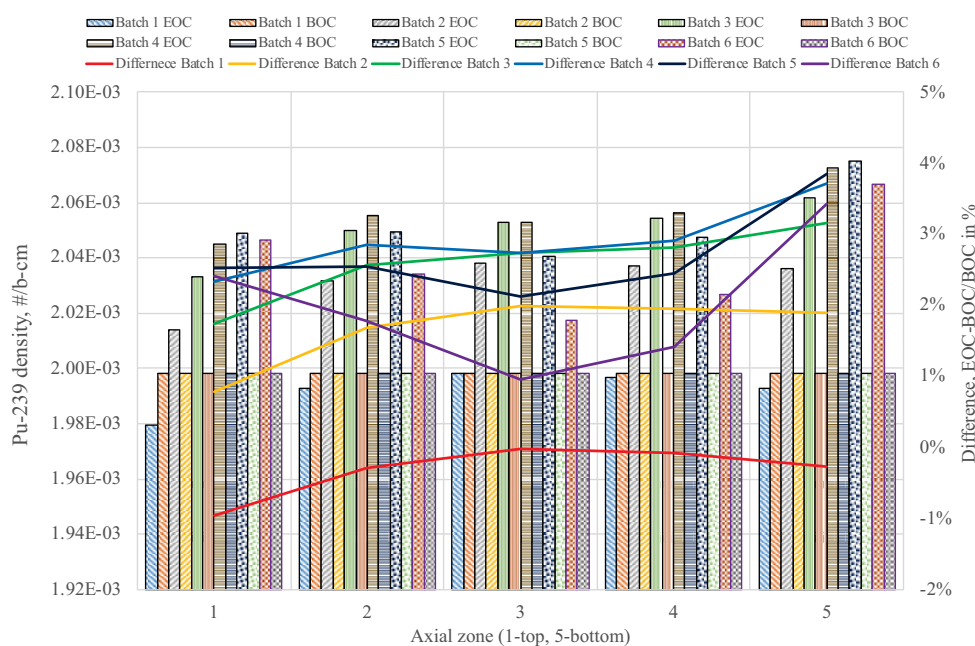
Figure 7: Plutonium concentration in inner fuel compared with BOL
