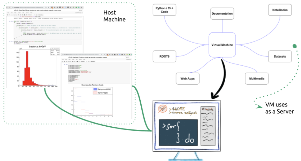
Figure 6. Schematic representation of how a VM is used to set a dedicated analysis suite for their users, allowing them to perform data analysis with Jupyter, not only to create and execute notebooks under several kernels (i.e. SaaS), but also as a simple IaaS by using the terminal provided by the Jupyter UI.
