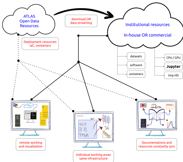
Figure 7. Schematic representation of a proposal on how users can access, run, and manipulate ATLAS Open Data resources in the cloud. From the use of university or institutional resources out of the HEP community (i.e. without previous access or knowledge to HEP software) and limited SysAdmins, or commercial clouds rented for a specific time by such universities or individuals running short-term workshops. A multi-user approach is implemented by design with as minimal setup as possible.
