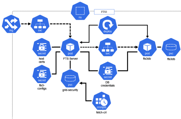
Fig. 2. Containerized configuration deployed in OKD
