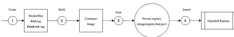
Fig. 1. Image registry workflow
