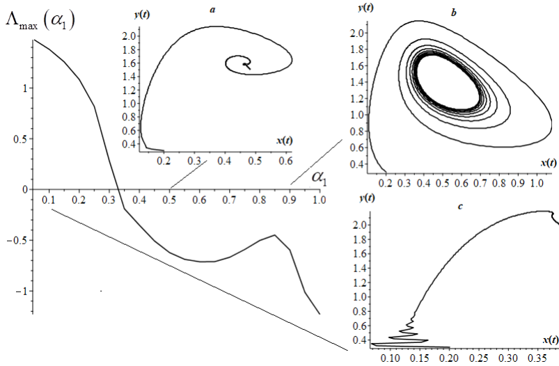
Figure 1. Spectrum of maximum Lyapunov exponents \Lambda_{\max}(\alpha_1) .
