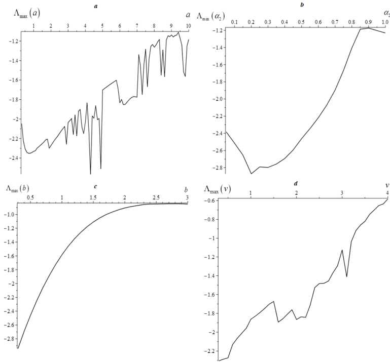
Figure 2. Spectra of maximum Lyapunov exponents: a – \Lambda_{\max}(a) , b – \Lambda_{\max}(\alpha_2) , c – \Lambda_{\max}(b) , d – \Lambda_{\max}(v) .
