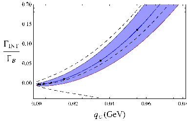
Figure 3. Ratio between the interference and the Bremsstrahlung contributions for the K^\pm \rightarrow \pi^\pm \pi^0 e^+ e^- decay. The solid line and the error bar correspond to the values displayed in the main text. The upper and lower dashed curves correspond to setting N_E^{(0)} = 0 and N_E^{(0)} = 0 , respectively. Figure borrowed from [6].
