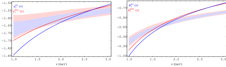
Figure 4. Scale dependence of the slope parameters a_+ and b_+ . Figure borrowed from [8].
