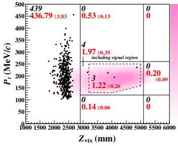
Figure 2. Data from the KOTO experiment for the period 2016-2018. All the data points are consistent with the background estimates. Figure borrowed from [5].
