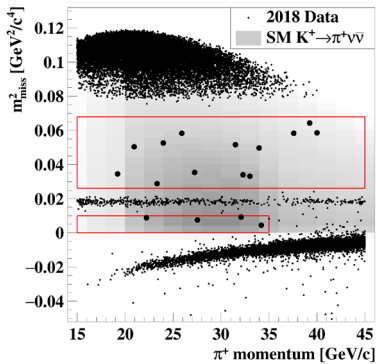
Figure 1. Kinematical details of the NA62 data for K^+ \rightarrow \pi^+ \bar{\nu} \nu corresponding to their 2018 dataset. Figure borrowed from [4].
