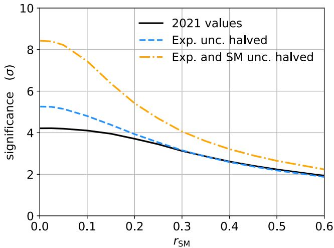
Figure 2. The significance of the muon g - 2 discrepancy as a function of r_{SM} assuming the 2021 uncertainties (with SM uncertainty from [3]), with the experimental uncertainty reduced by a factor of two, and with the SM uncertainty also halved.
