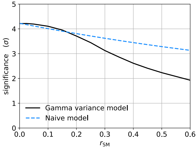
Figure 1. The significance of the muon g - 2 discrepancy as a function of the relative uncertainty r_{\text{SM}} in the quoted systematic uncertainty of the SM prediction (the relative “error on the error”).
