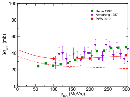
Figure 3. Annihilation cross section for \bar{n}p scattering multiplied with the velocity \beta of the incoming antineutron. The curves show the results for the N^3LO interaction with cutoff radius R = 0.9 fm [4]. The dashed line is the contribution from the {}^3S_1 - {}^3D_1 partial wave while the solid line is the full result. Data are from Refs. [34, 36].
