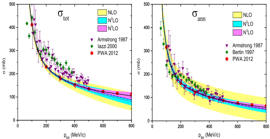
Figure 2. Total ( \sigma_{tot} ) and integrated annihilation ( \sigma_{ann} ) cross sections for \bar{n}p scattering. Same description of curves and bands as in Fig. 1. Data are from Refs. [34–36].
