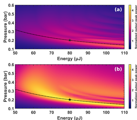
Figure 1. Peak power of the self-compressed pulses normalized to its initial value as a function of input pulse energy and equivalent gas pressure for (a) a statically argon-filled HCF and (b) its equivalent differentially pumped fiber with a decreasing pressure gradient. The dot-dashed line represents the curve of constant B-integral ( B = 8.5 rad) which best fits the optimal region for high-quality self-compression and the star refers to the final situation shown in Fig. 2 (80 \mu J, 200 mbar).
