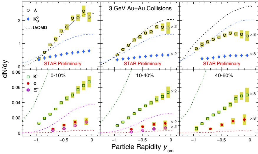
Figure 1. The rapidity dependence of dN/dy of \Lambda , K_S^0 , K^- , \phi and \Xi^- in Au+Au collisions at \sqrt{s_{NN}} = 3 GeV in different centralities. The yields at 10-40% and 40-60% are scaled up by a factor of 2 and 8 respectively for better visibility. The vertical lines and bands represent the statistical and systematic uncertainties. The dashed lines are the calculations from UrQMD.
