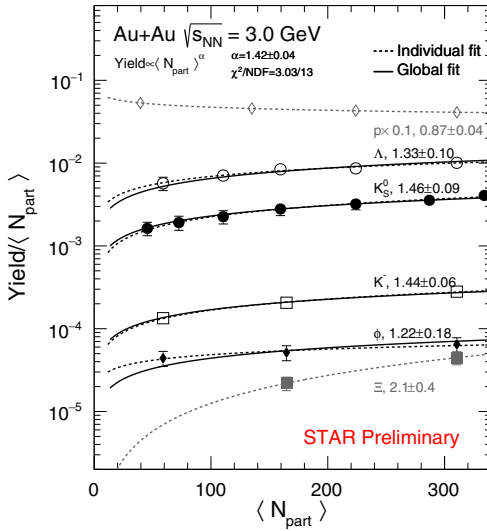
Figure 3. Hadron yields per mean number of participants as a function of \langle N_{part} \rangle . All hadron yields are fitted with a function of the form f \propto C \langle N_{part} \rangle^\alpha shown as black dash lines, and the fitted \alpha values are shown in the figures. The black solid lines represent a simultaneous fit to all strange hadron yields ( K^- , K_S^0 , \Lambda , \phi ).
