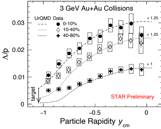
Figure 2. Rapidity dependence of \Lambda/p for different centrality bins in Au+Au collisions at \sqrt{s_{NN}} = 3 GeV. Vertical lines represent statistical uncertainties, while boxes represent systematic uncertainties. 10-40% centrality is shifted left for better visibility. The curves represent the calculations from UrQMD and are scaled up to compare with data.
