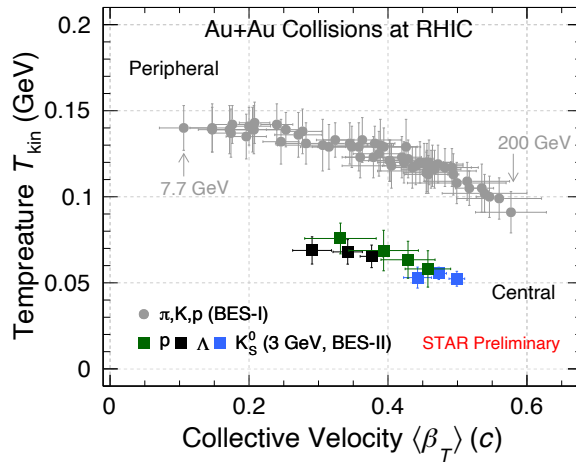
Figure 4. Effective temperature T_{kin} vs collective velocity \langle\beta_T\rangle for p (green), \Lambda (black) and K_S^0 (blue) extracted from blast-wave fits at \sqrt{s_{NN}} = 3 GeV. The fit parameters for (\pi, K, p) from \sqrt{s_{NN}} = 7.7 to 200 GeV are shown for comparison.
