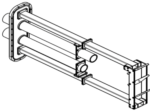
Figure 1. Two quasi-optical system for ECE front end
