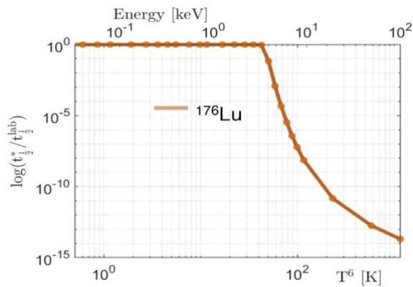
Fig. 4 – Theoretical prediction of stellar half-life to terrestrial half-life ratio for ^{176}\text{Lu} nucleus as a function of plasma temperature expressed in T^6 [ 10^6\text{ K} ] (Energy [keV]). Calculations were performed at plasma densities of 10^{12}\text{ cm}^{-3} .
