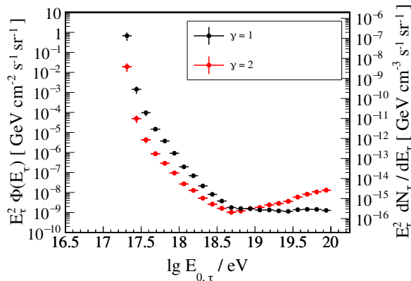
Figure 8. Differential upper limits on the isotropic emergence of \tau leptons near the ground at 95 % confidence level. The left axis corresponds to the flux of \tau -leptons created within 50 km of path length below the Earth's surface, and the right scale shows the limits on the rate of \tau s generated per unit volume, energy, and solid angle. Two indicated spectral indices of the \tau flux are assumed.
