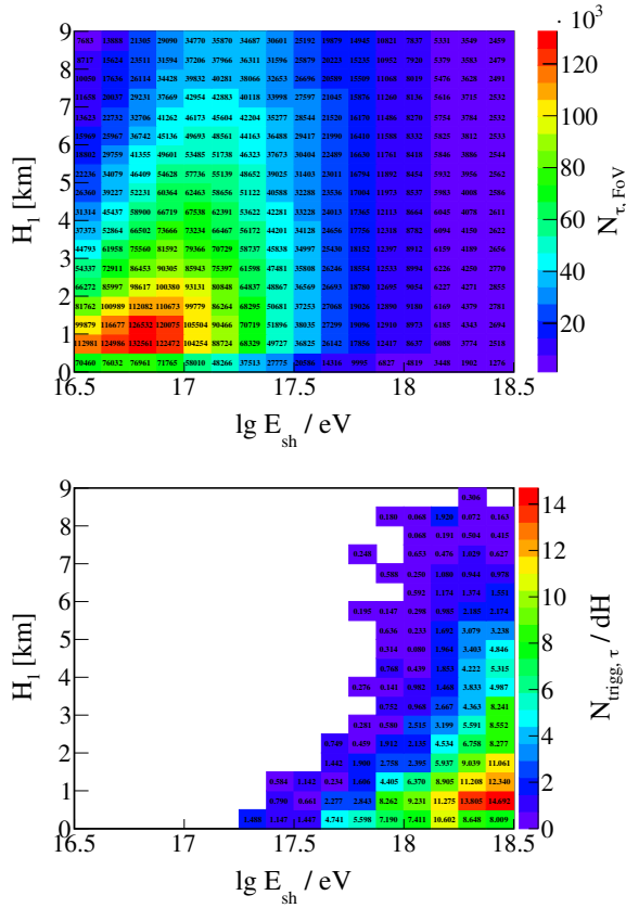
Figure 7. Distribution of MC-generated \tau -decay induced EAS within the FoV of the FD (top panel) and corresponding number of FD-triggered events per height bin (bottom panel). The height H_1 corresponds to the distance D_1 in Fig. 6 and coincides with H_{\text{fl}} .
