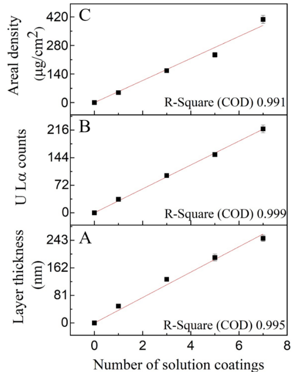
Fig 2. Number of solution coatings in function of layer thickness (A), U La counts (B) and areal density (C) derived from SEM, XRF and α-particle spectroscopy measurements, respectively. It is shown that the uranium content in the targets increases linearly with increasing number of coatings of the solutions.
