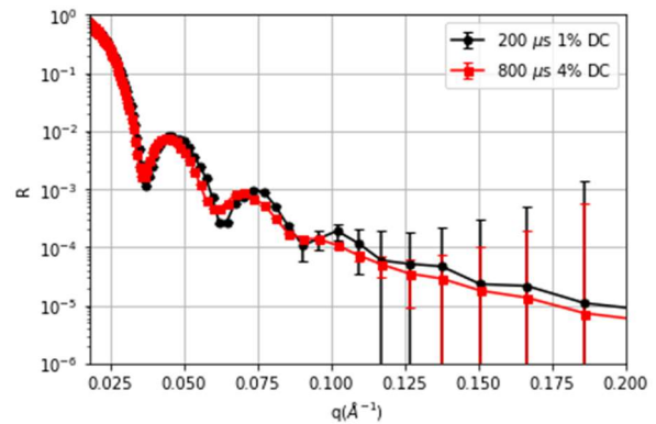
Fig. 9. Simulated reflectivity curve for a 20 nm Ni layer on Si for different pulse lengths.
