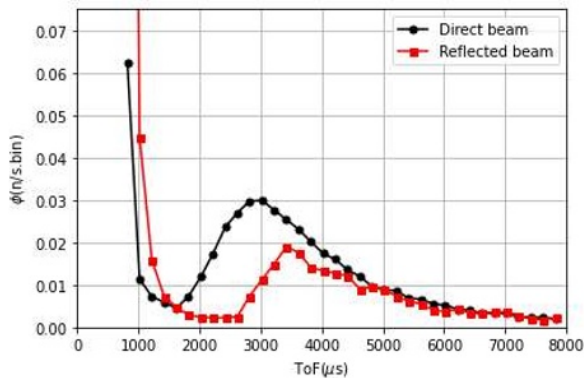
Fig. 10. Direct beam and reflected beam by an m = 4 supermirror measured at HERMES (bin size: 200 \mu\text{s} ).
