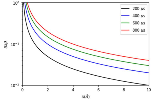
Fig. 8. Wavelength resolution for different pulse lengths.
