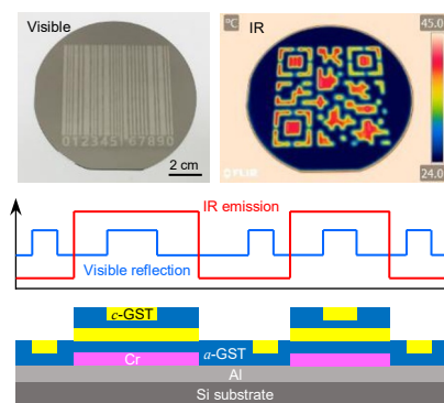
Fig. 1. Structure of a GST cavity fabricated on a Si substrate along with its visible and IR images. a -GST represents amorphous GST and c -GST refers to crystalline GST.
