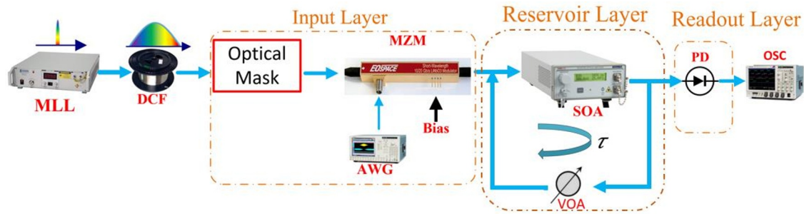
Fig. 1: The schematic of the proposed all-optical reservoir computer. MLL: Mode-Locked Laser, DCF: Dispersion Compensating Fibre, MZM: Mach-Zehnder modulator, AWG: Arbitrary Waveform Generator, VOA: Variable Optical Attenuator, SOA: Semiconductor Optical Amplifier, PD: Photodetector, OSC: Oscilloscope.
