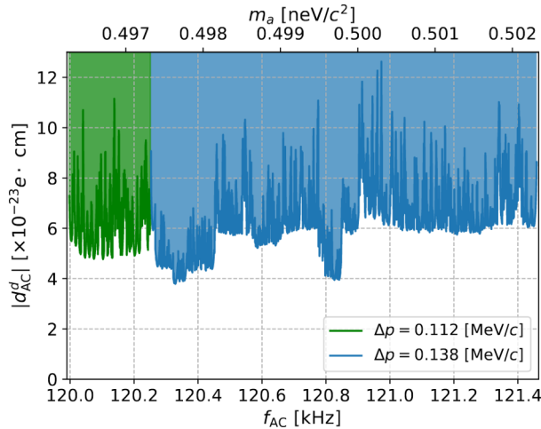
Figure 6. Preliminary 90% upper confidence level sensitivity for excluding the ALPs induced oscillating deuteron EDM in the frequency range from 120.0 to 121.4 kHz and the corresponding axion mass range of 4.95 to 5.02 \times 10^{-9} eV. The green and blue colors show two scanning ramp rates in momentum change. The darker lines denote the upper bounds on the oscillating EDM, the shaded area is the excluded region. Figure taken from [17].
