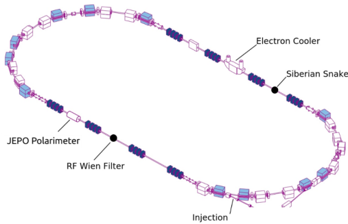
Figure 2. The schematic of Cooler Synchrotron COSY showing the positions of the principal elements.
