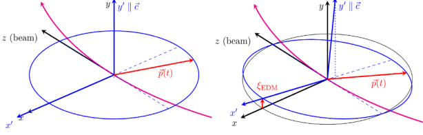
Figure 4. Invariant spin axis is vertical in case of an ideal ring in the absence of the EDM (left), tilted in radial direction due to EDM effect (right). Figure is taken from [2].
