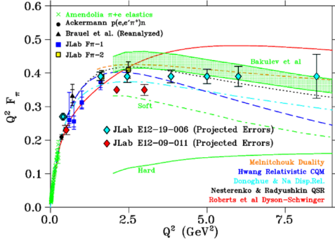
Figure 6. Expected statistical and systematic uncertainties on the pion elastic form factor from Hall C, from the reaction e^-p \rightarrow e^-\pi^+n . The analysis requires that the longitudinal and transverse components of the cross section be separated, and a model used to extract F_\pi from the magnitude and t -dependence of the longitudinal component. This difficult measurement will extend the Q^2 range by more than a factor of two over existing data, owing to the high reach afforded by 12 GeV CEBAF.
