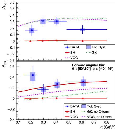
Figure 5. Measurement from CLAS12 [9] of the photon polarization asymmetry A_{0U} (top) and the forward-backward asymmetry A_{FB} (bottom) in Timelike Compton Scattering from the proton compared to models. The Bethe-Heitler process predicts only very small asymmetries, clearly inconsistent with the data. Good agreement with models is obtained for A_{0U} , which is primarily sensitive to the imaginary part of the Compton Form Factor \mathcal{H} . On the other hand, good agreement with A_{FB} , which is sensitive to the real part of \mathcal{H} , requires inclusion of the so-called D -term which has recently gained relevance for its links to the mechanical properties of the nucleon.
