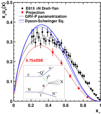
Figure 7. Data on the \pi^- valence quark distribution function from the reaction \pi^-A \rightarrow \mu^+\mu^-X on a Be target [10] compared to models based on the Dyson-Schwinger Equations [11] and next to leading order QCD resummation [12]. The inset shows a different experimental approach based on the Sullivan process, where one carries out deep inelastic scattering on the pion cloud of the nucleon. This approach is the basis of the Tagged Deep Inelastic Scattering (TDIS) experimental program planned for CEBAF, as well as the Electron Ion Collider (EIC).
