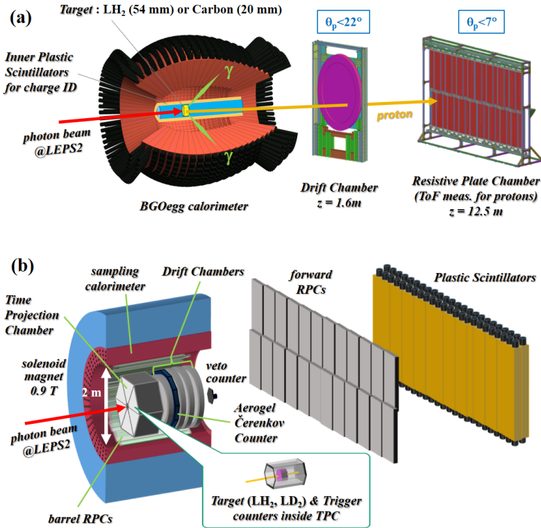
Figure 1. Two detector setups for hadron photoproduction experiments in SPring-8 LEPS2 project. (a) and (b) show the detector systems for BGOegg experiment and LEPS2/Solenoid experiment, respectively.
