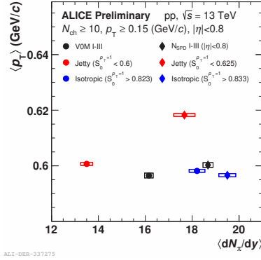
Figure 2: Correlation between \langle p_T \rangle and \langle dN_\pi/dy \rangle as a function of S_0^{p_T=1} , in the 0–10% VOM and N_{Tracklets} multiplicity classes.
