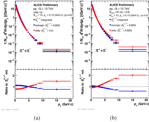
Figure 3: The pion transverse momentum spectra obtained in 0–10% multiplicity class in (a) VOM and (b) N_{\text{Tracklets}} for pp collisions at \sqrt{s} = 13 TeV for two spherocity classes and S_0^{p_T=1} -integrated class.
