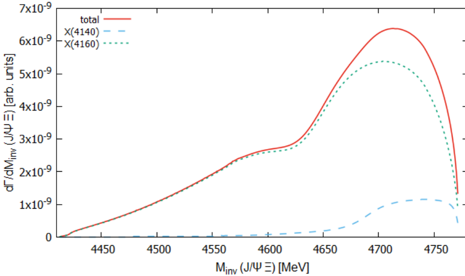
Figure 3. The red line represents the J/\psi \Xi spectrum computed with a narrow X(4140) plus a X(4160) , while the blue and the green ones show the individual contribution from the X(4140) and the X(4160) , respectively.
