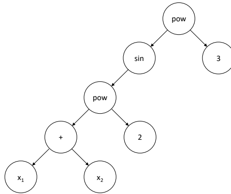
Figure 1. The tree-like representation of the expression \sin^3[(x_1 + x_2)^2] .
