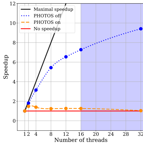
Figure 2. Speedup versus number of threads after implementing thread safety. The black solid curve shows the ideal case with linear maximal speedup, while the red solid horizontal curve shows no speedup. The dotted blue curve shows the large increase in code execution speed when FSR is not enabled (PHOTOS off), while the dashed orange curve shows the limited speedup when FSR is enabled (PHOTOS on). The blue shaded area corresponds to the hyperthreading regime.
