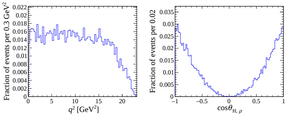
Figure 1. Examples of validation histograms. Left: distribution of dimuon invariant-mass squared m(\mu^+\mu^-)^2 = q^2 (in natural units c = 1 ) for B^+ \rightarrow K^+\mu^+\mu^- decays simulated with the BTOSLLBALL decay model. Right: distribution of helicity angle \cos \theta_{H,\rho} for B^+ \rightarrow \bar{D}^0\rho^+(\rightarrow \pi^+\pi^0) decays simulated with the SVS decay model. The helicity angle \cos \theta_{H,\rho} corresponds to the angle between the B^+ and the \pi^+ momenta in the \rho^+ frame.
