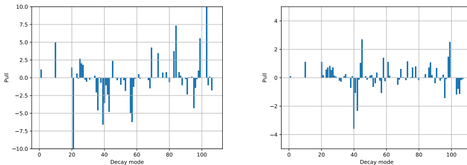
Figure 4. Pulls of branching fractions for known D_s^+ decay modes (left) before and (right) after updating the decay table database as described in the text. Note the different scales on the y -axis.
