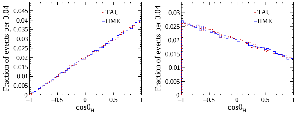
Figure 3. Distributions of helicity angle \cos \theta_H for simulated (left) B^+ \rightarrow \tau^+(\rightarrow \pi^+ \bar{\nu}_\tau) \nu_\tau and (right) B^+ \rightarrow \tau^+(\rightarrow \mu^+ \nu_\mu \bar{\nu}_\tau) \nu_\tau decays. The helicity angle \cos \theta_H corresponds to the angle in the \tau frame between the B^+ and the \pi^+ for the left plot, and between the B^+ and the \mu^+ for the right plot. The solid blue (dotted red) curve corresponds to events where the \tau decays are simulated with the Pythia HME module (TAUOLA generator).
