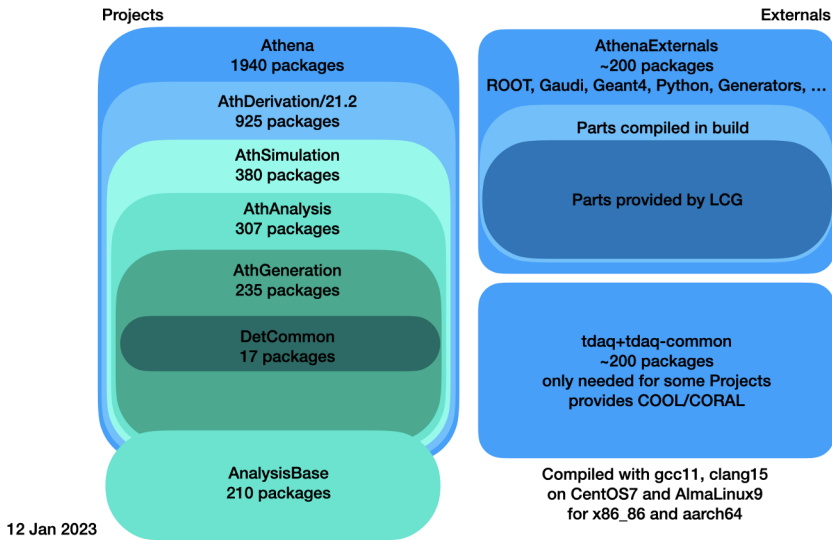
Figure 1: Overview of the building blocks of the ATLAS experimental software.
