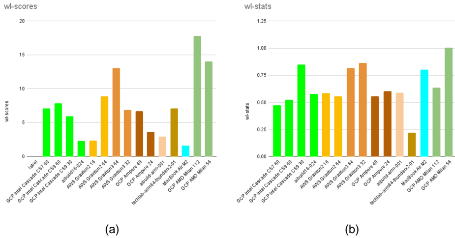
Figure 3: (a) HEPscore results for the ATLAS reconstruction work ow and (b) a single work ow with four CPU threads only. Larger values of wl-scores and wl-stats are better. ARM type CPUs coloured brown, orange and blue and are grouped in the middle of both plots as bars 5–13. The x86_64 type CPUs are at the very left and right of the plots and coloured green.
