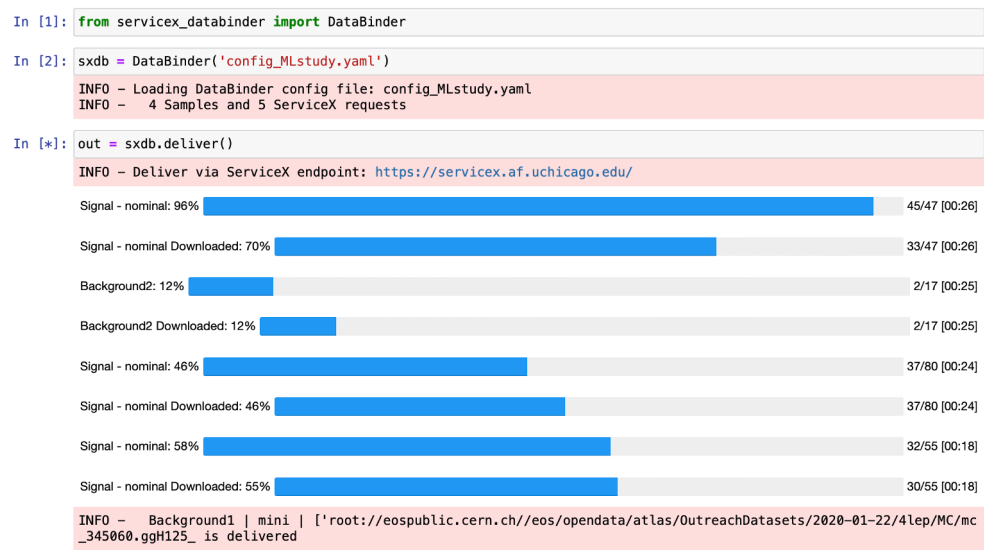
Figure 3. An example of running servicex-databinder in a Jupyter notebook.
