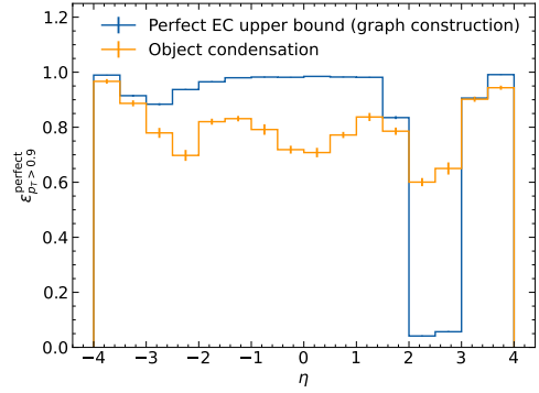
Figure 3: An OC pipeline outperforms a perfect EC when edges between the barrel and the right endcap have been removed.
