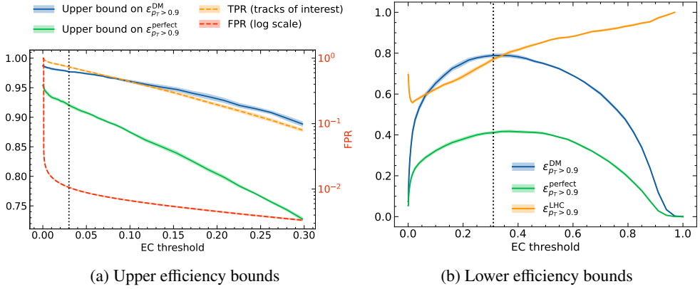
Figure 1: Performance of the edge classifier applied during edge construction. The left plot shows the true positive and false positive rates together with approximate upper bounds on the recoverable performance based on a perfect EC. The right plot shows the achievable tracking performance by applying a cut on the edge classifier and identifying tracks with connected components of the resulting subgraph. Note that \epsilon_{p_T>0.9}^{\text{DM}} is not strictly monotonous because it is normalized to the number of reconstructed tracks rather than particles.
