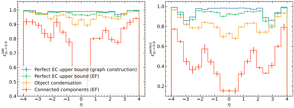
Figure 5: Comparing the performance of the OC pipeline with the upper and lower bounds introduced in this paper.
