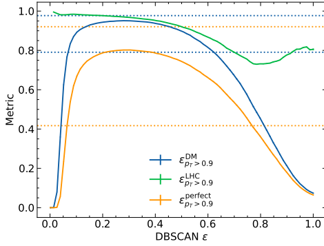
Figure 2: Optimizing the DBSCAN hyperparameters to obtain the maximum performance. The dashed lines are the upper and lower bounds after the EF step for reference (see Figure 1).
