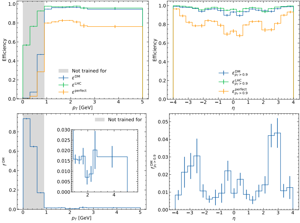
Figure 4: Tracking performance in bins of p_T and \eta .
