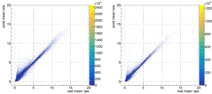
Figure 4. The 2D scatter plot shows the target (or real) expected N p.e. (in the X-axis) versus the predicted value (in the Y-axis) for HighQENNV PMTs (left) and Hamamatsu PMTs (right)
