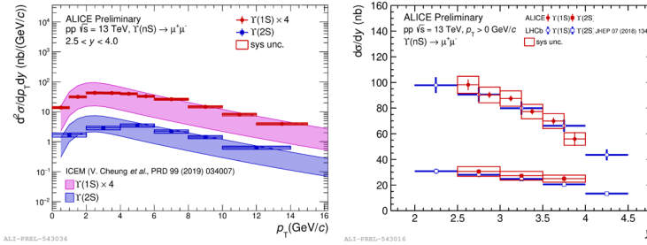
Figure 2. (Left) Inclusive \Upsilon(1S) and \Upsilon(2S) cross sections, at forward y , as a function of p_T , measured in pp collisions at \sqrt{s} = 13 TeV. The data are compared with theoretical calculations from ICeM + FONLL [8, 9]. (Right) Rapidity dependence of inclusive \Upsilon(1S) and \Upsilon(2S) cross sections, at forward y , measured in pp collisions at \sqrt{s} = 13 TeV. The results are compared with LHCb measurements at the same center-of-mass energy [10].
