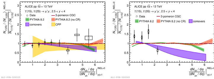
Figure 3. Self normalized (left) \Upsilon(2S) -to- \Upsilon(1S) and (right) \Upsilon(3S) -to- \Upsilon(1S) yield ratios, at forward y , as a function of self-normalized charged-particle multiplicity at midrapidity in pp collisions at \sqrt{s} = 13 TeV. The measurements are compared with PYTHIA 8.2 event generator, 3-pomeron-CGC, CPP, and comover models. Model descriptions can be found in [11].
