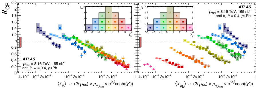
Figure 1. R_{CP} as a function of approximated longitudinal momentum fractions x_p (left panel) and x_{Pb} (right panel) [4]. Shaded rectangles and vertical error bars represented the systematic and statistical uncertainty, respectively. Solid rectangles on the left-side stand for the uncertainty on the T_{AB} .
