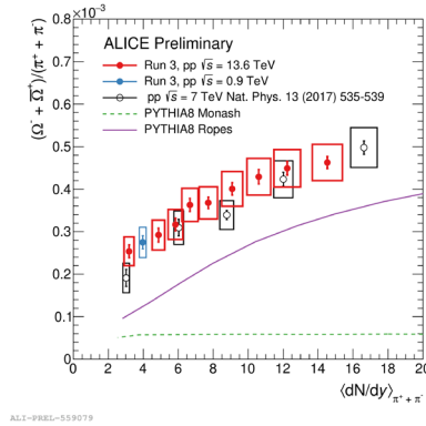
Figure 3. \Omega^- + \bar{\Omega}^+ to pion yield ratio as a function of the charged-pion multiplicity for different FT0M multiplicity classes at \sqrt{s} = 13.6 TeV and for the inclusive INEL > 0 sample at \sqrt{s} = 900 GeV.
