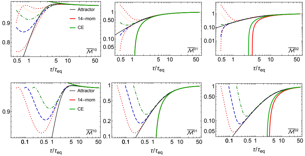
Figure 1. Scaled moments \overline{\mathcal{M}}^{nl} as a function of rescaled time for the case m = 1 GeV and T_0 = 1 GeV. The solid black lines correspond to the attractor solution, the solid red lines are the first-order 14-moment predictions in eq. (8), and the solid green lines are the first-order Chapman-Enskog predictions in eq. (9). Top: The non-solid lines are specific initial conditions initialized at \tau_0 = 0.1 fm/c with \alpha_0 = 1/\sqrt{1+\xi_0} \in \{0.12, 0.25, 0.5, 1, 2\} . Bottom: the non-solid lines are specific initial conditions initialized with \xi_0 = 0 at \tau_0 \in \{0.01, 0.02, 0.04\} fm/c. Note that for \overline{\mathcal{M}}^{10} and \overline{\mathcal{M}}^{01} , the 14-moment and Chapman-Enskog predictions are the precisely the same.
