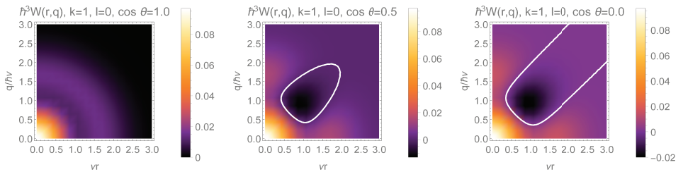
Figure 1. Phase-space distribution W_{10} for quantum numbers k = 1, l = 0 as functions of r = |\mathbf{r}| and q = |\mathbf{q}| . The white lines indicate nodes where W_{10} = 0 . Distributions are shown for several values of the angle \theta given by \cos \theta = \mathbf{r} \cdot \mathbf{q} / r q .
