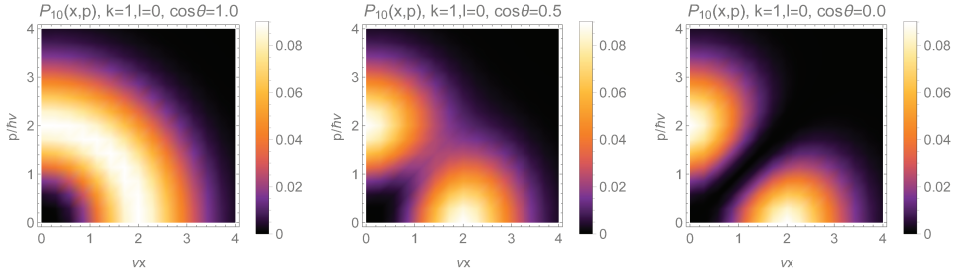
Figure 2. Coalescence probabilities \mathcal{P}_{10} for quantum numbers k = 1, l = 0 for two Gaussian wave packets being mutually attracted by an isotropic 3-D harmonic oscillator potential. Probabilities are shown as functions of relative coordinates x = |\mathbf{x}| and p = |\mathbf{p}| for several values of the angle \cos \theta = \mathbf{x} \cdot \mathbf{p} / xp between the vectors.
