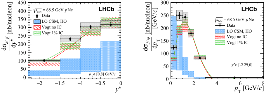
Figure 3. The differential cross sections for J/\psi production in p Ne collisions as a function of the J/\psi (left) y^* and (right) p_T [4]. The LHCb data points in black are compared to several theoretical models (see text for details).
