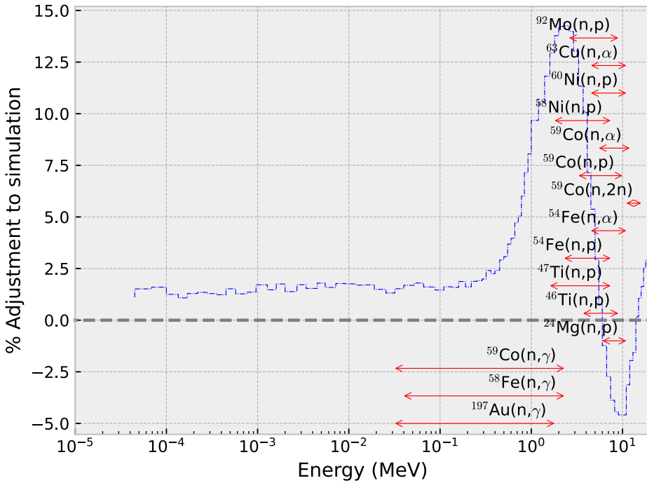
Fig. 6. Adjustment to simulation, STAYSL_PNNL output versus MCNP6.2 using ENDF/B-VIII.0 with 10%/90 % reaction activity bands illustrated.
