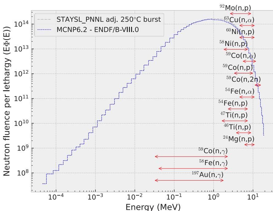
Fig. 5. STAYSL_PNNL adjusted spectrum and a priori spectrum from MCNP6.2 using ENDF/B-VIII data with 10%/90 % reaction activity bands illustrated.
