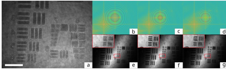
Figure 2. Examples of hologram reconstruction for 3 distances with the corresponding phase propagators. The sub-figure a correspond to an experimental off-axis digital hologram of a USAF 1951 resolution test chart. Sub-figures b , c and d represent the simulated digital propagators of the hologram for the reconstruction distances -54\ \mu\text{m} , -74\ \mu\text{m} and -94\ \mu\text{m} respectively. The sub-figures e , f and g correspond to the numerical reconstruction in amplitude of the off-axis hologram at the distance -54\ \mu\text{m} , -74\ \mu\text{m} and -94\ \mu\text{m} respectively. In the sub-figures b , c and d , the yellow peaks correspond to the 0 and +1 orders of the spectrum and the wrapped rings to the phase propagator, the propagator is centred on the +1 order. SLED@ \lambda = 650\ \text{nm} , bandwidth \Delta\lambda = 6\ \text{nm} . Scale bar: 100\ \mu\text{m}
