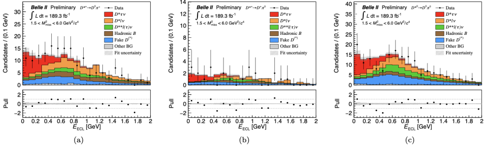
Figure 1. Distributions of E_{ECL} in the signal-enhanced region 1.5 < M_{miss}^2 < 6.0 GeV^2/c^4 for the D^{*+} \rightarrow D^0 \pi^+ (left), D^{*+} \rightarrow D^+ \pi^0 (middle), and D^{*0} \rightarrow D^0 \pi^0 (right) modes, with fit projections overlaid. The bottom panel presents pull values from fit results. The rectangular-shaded regions on the histograms and in the pull plot correspond to statistical uncertainties in the fit.
