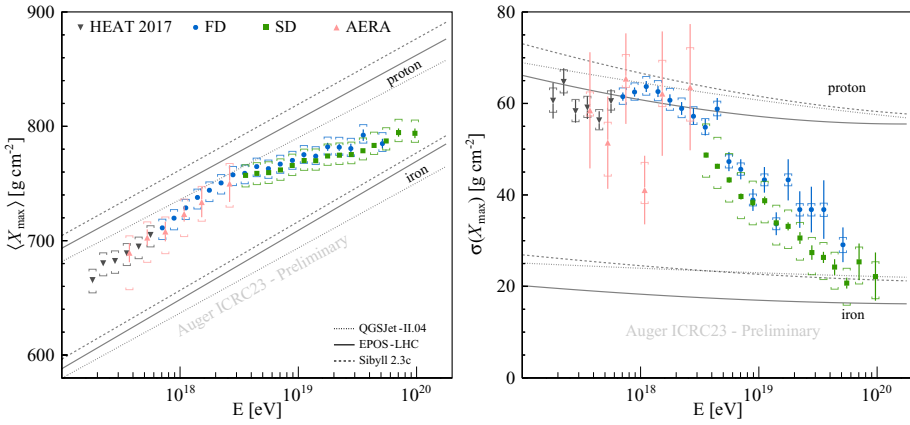
Figure 2. Energy evolution of the average (left) and standard deviation (right) of X_{\max} distribution. Data from horizontally-looking telescopes are marked as FD [7] while high-elevation data as HEAT 2017 [10]. The estimate from deep learning is given as SD [9], and AERA shows the radio dataset [8]. Reproduced from Ref. [11].
