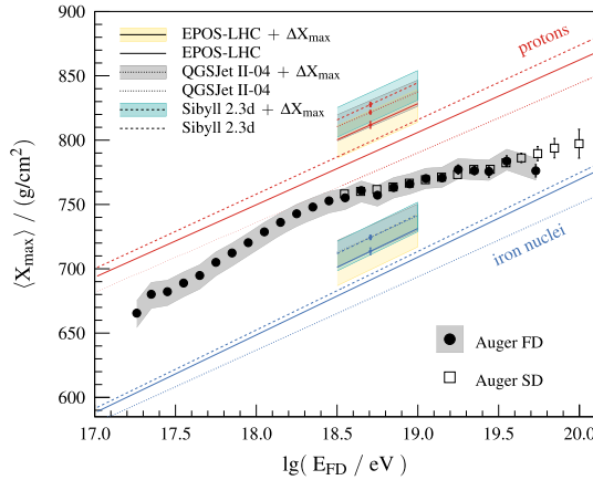
Figure 3. Average X_{\max} measured at the Pierre Auger Observatory accompanied by predictions of unmodified (without bands) and modified (with bands) models of hadronic interactions. The X_{\max} modifications are needed to describe the FD and SD data together. Bands correspond to systematic uncertainties. Taken from Ref. [12].
