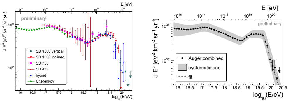
Figure 1. The energy spectrum of cosmic rays derived from six data sets of the Pierre Auger Observatory (left) and the combined spectrum (right). Data come from Refs. [4, 5].
