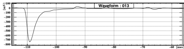
Figure 4. Typical waveform of the prototype detector irradiated with \beta -rays. From the signal size, it is most likely a 3 photoelectron event.
