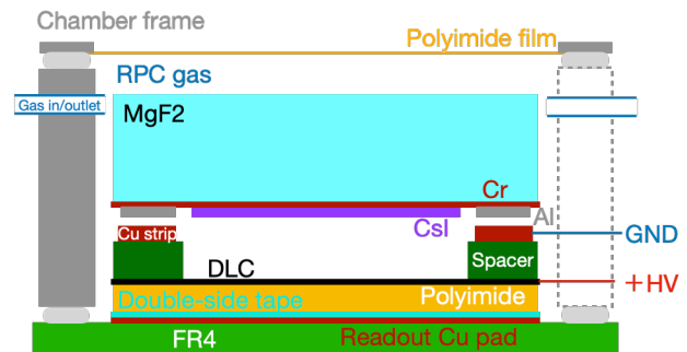
Figure 3. Schematic view of the prototype detector (not to scale)
