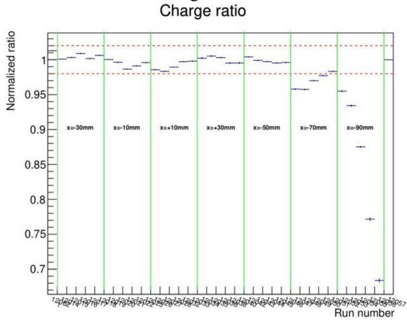
Fig. 7. Normalized ratio between the low and the high light channel as a function of different incident positions of the beam on the calorimeter.
