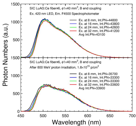
Fig. 3. PL spectra of the \phi 1 \times 40 \text{ mm}^3 LuAG:Ce ceramic fiber #6 measured before (top) and after (bottom) 1.8 \times 10^{15} \text{ p/cm}^2 .
