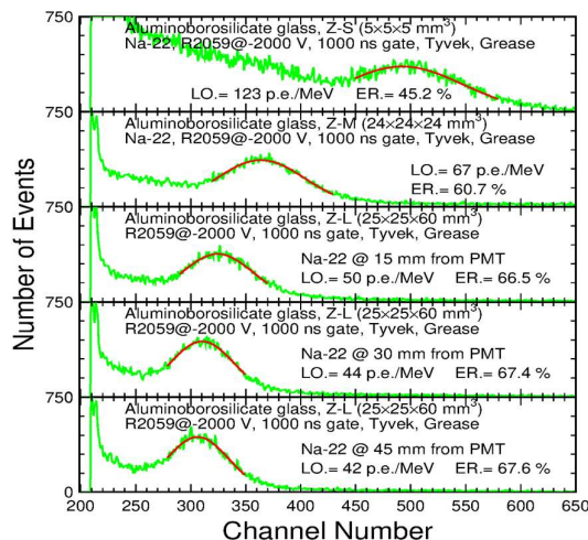
Fig. 11. PHS measured with one μs gate is shown for the three ABS glass samples.
