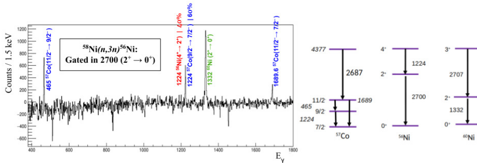
Figure 2. Prompt \gamma spectrum, gated on 2700 keV, showing the evidence of ^{56}\text{Ni} along with other contributions.
