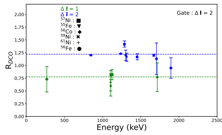
Figure 4. Measured DCO ratios for known dipole and quadrupole transitions using gates on stretched quadrupoles.
