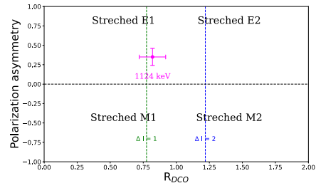
Figure 5. Asymmetry ratio as a function of the DCO ratio for the transition from the 3701 keV state in ^{57}\text{Ni} .
