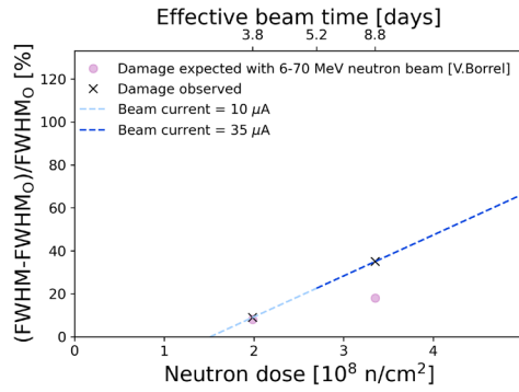
Figure 1. The evolution of degradation with neutron dose, as observed for the 1332 keV line of ^{60}\text{Co} , is shown. The fits performed are linear, based on only two data points, which describe the behavior of the relative FWHM.
