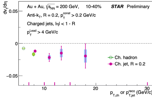
Figure 2: Measurement of the slope of jet (magenta solid circles) and charged-hadron (green open circles) v_1 versus pseudorapidity, as a function of p_T in Au+Au collisions.
