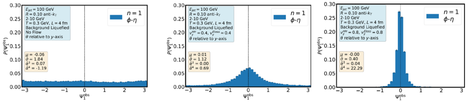
Figure 3. The distribution of dipole angles \{\psi_i\} in the \eta - \phi plane for jets as defined in the text. Jets without flow (left panel), with transverse flow velocity v = 0.4 during (center panel) and transverse flow velocity v = 0.8 (right panel) are shown. In the center and right panel the flow angle \psi_F is set to be zero and therefore the observed dipole angles are highly correlated with the flow angle.
