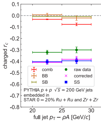
Figure 3. r_c from various contributions for two selections of background subtracted jet p_T .
