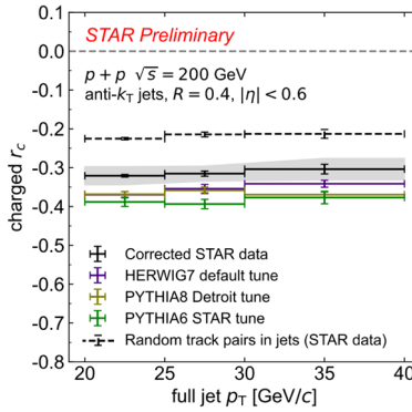
Figure 1. r_c as a function of jet p_T in p+p collisions, for the fully corrected STAR data (black solid), with comparison with predictions from HERWIG7 [6] (purple), PYTHIA8 [7] Detroit tune [8] (gold) and PYTHIA6 [9] STAR tune [10] (green). Effective r_c for random track pairs in jets in STAR data is shown in black dashed lines.
