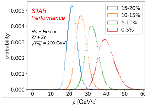
Figure 2. \rho distribution for isobar collision events, with centralities of 0 – 5% (red), 5 – 10% (green), 10 – 15% (orange), and 15 – 20% (blue).
