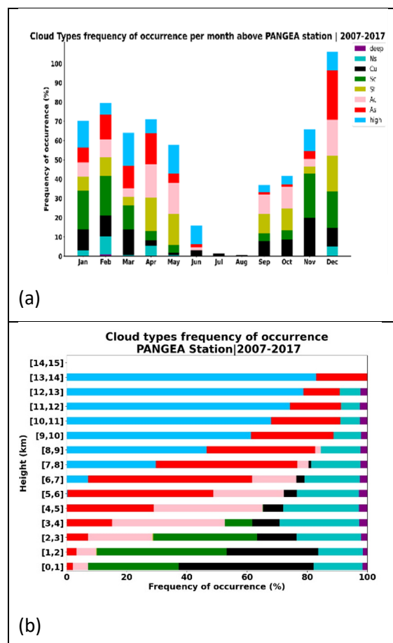
Figure 1. Frequency of cloud type occurrence (a) per month, and (b) per height from CloudSat for the period 2007 to 2017.
