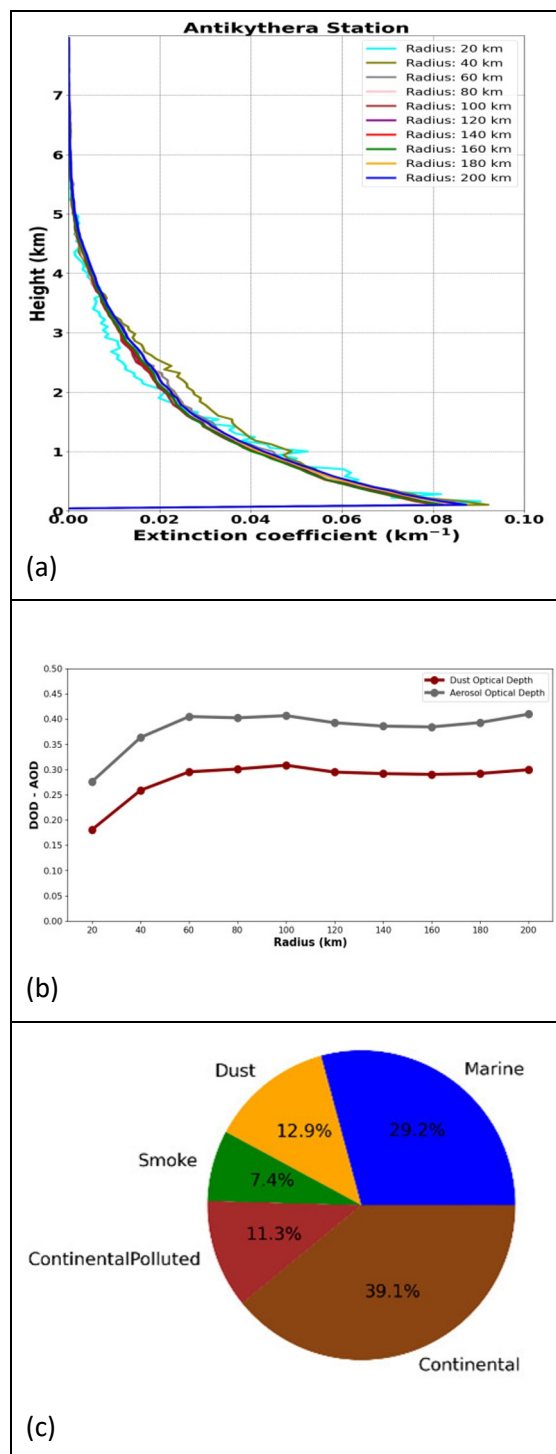
Figure 1. Total Aerosol Mean Extinction coefficient profiles at 532 nm (a) and AOD and DOD (b) for different radii around PANGEA site for the period between June 2006 and December 2021, using LIVAS dataset. Percentages of the detected aerosol layer types over PANGEA from 1 year of lidar measurements (c).
