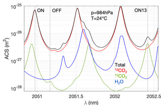
Figure 1. Absorption cross-section (ACS) for ^{12}\text{CO}_2 , ^{13}\text{CO}_2 and \text{H}_2\text{O} for pressure 984 hPa and temperature 24°C. \text{H}_2\text{O} ACS have been multiplied by a factor of 25 with respect to mixing ratios in the atmosphere ( \text{CO}_2 : 0.04%, \text{H}_2\text{O} : 1%). ^{13}\text{CO}_2 ACS is multiplied by the VPDB isotopic ratio. The DIAL wavelengths for OFF, ON and ON13 positions are indicated.
