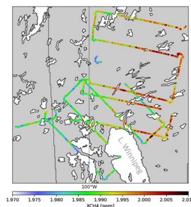
Figure 4. Enhancements of the methane column in ppm measured by CHARM-F over the wetlands north-east of Lake Winnipeg, Manitoba, along two HALO flights.
